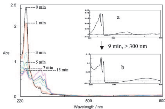
Fig. 7. Photolysis ( \lambda > 300 \text{ nm} ) of diazide 2b in solid Ar at 13 K. UV spectra (a) before irradiation; (b) after 1 min of irradiation; (c) after 3 min of irradiation; (d) after 5 min of irradiation; (e) after 7 min of irradiation; (f) after 15 min of irradiation. In inset is the difference UV spectra after (a) 2 and (b) 11 min of irradiation.
