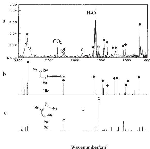
Fig. 9. (a) IR spectrum after irradiation ( \lambda > 300 nm, 9 h) of diazide 2c in Ar at 13 K. Theoretical (B3LYP/6-31G*) IR spectra of 10c (b) and 9c (c).
