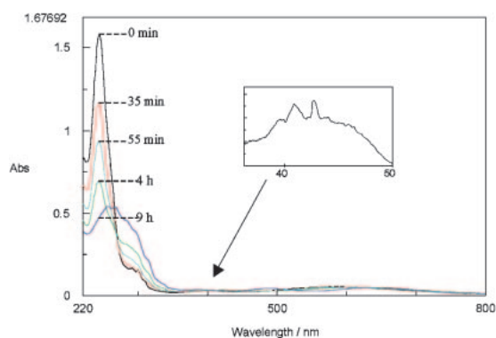
Fig. 4. Photolysis ( \lambda > 300 nm) of diazide 2a in solid Ar at 13 K. UV spectra (a) before irradiation; (b) after 35 min of irradiation; (c) after 55 min of irradiation; (d) after 4 h of irradiation; (e) after 9 h of irradiation. In the inset is the difference UV spectrum after 20 min of irradiation.
