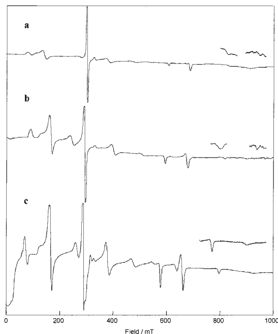
Fig. 1. EPR spectra after irradiation ( \lambda > 300 \text{ nm} , 2MTHF, 77 K) of diazide 2a ( \nu_0 = 9.243 \text{ GHz} ) (a), diazide 2b ( \nu_0 = 9.212 \text{ GHz} ) (b), and diazide 2c ( \nu_0 = 9.231 \text{ GHz} ) (c).
