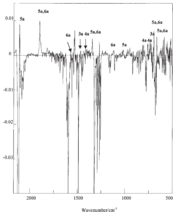
Fig. 2. Difference spectrum before and after irradiation ( \lambda > 300 \text{ nm} , 1 min) of diazide 2a in Ar at 13 K.
