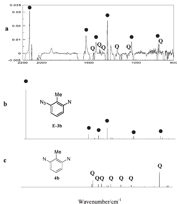
Fig. 5. (a) Difference spectrum before and after irradiation ( \lambda > 245 \text{ nm} , 2 min) of diazide 2b in Ar at 13 K. Theoretical (UB3LYP/6-31G*) IR spectra of triplet E - 3b (b), and quintet 4b (c).
