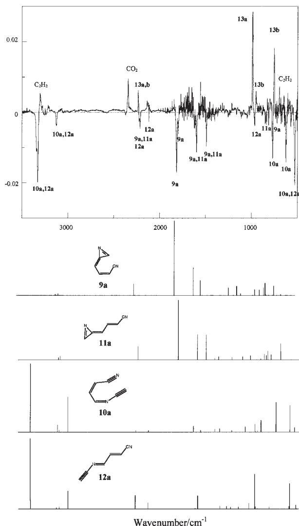
Fig. 3. Difference IR spectrum from photolysis ( \lambda > 270 nm, 3 h) of 2a in Ar at 13 K and theoretical (UB3LYP/6-31G*) IR spectra of 9a , 11a , 10a , and 12a .
