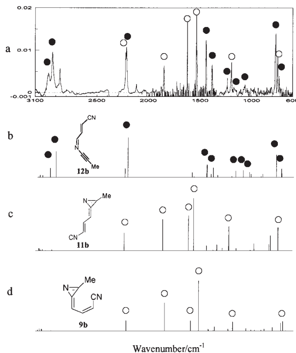
Fig. 6. (a) IR spectrum after irradiation ( \lambda > 300 nm, 3 h) of diazide 2b in Ar at 13 K. Theoretical (B3LYP/6-31G*) IR spectra of 12b (b), 11b (c), and 9b (d).
