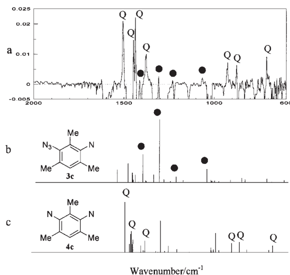
Fig. 8. (a) Difference spectrum before and after irradiation ( \lambda > 300 \text{ nm} , 30 min) of diazide 2c in Ar at 13 K. Theoretical (UB3LYP/6-31G*) IR spectra of triplet 3c (b), and quintet 4c (c).
